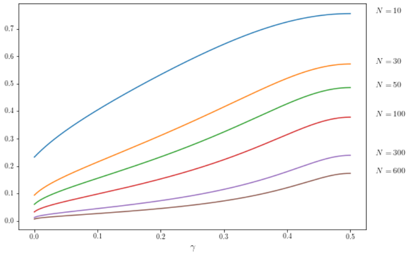
FIGURE 4. Total turnout rate as a function of \gamma using different values of N . Cost distribution Log-normal (-0.88, 0.8) .
