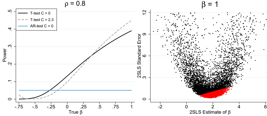
Figure 3. Power of the T-Test vs. AR-Test when Model is Not Identified ( C = 0 )
