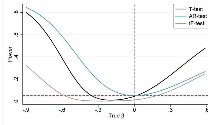
Figure 6. Power of the tF , t and AR Tests ( C = 10 , \rho = 0.5 )
