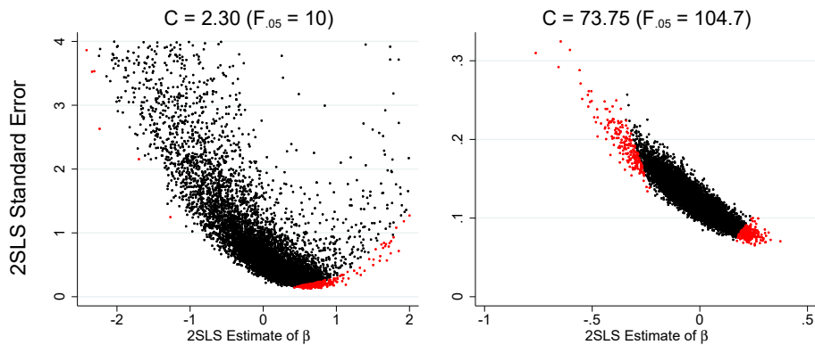
Figure 4. AR-test rejections: SE(\hat{\beta}_{2SLS}) plotted against \hat{\beta}_{2SLS} ( \rho = 0.80 )
